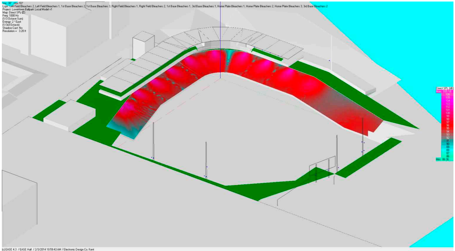
Acoustical 3D Modeling-Bowl Coverage
